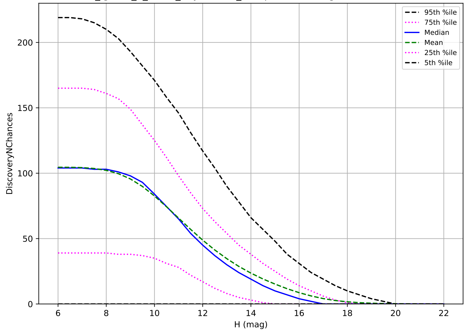
too_ignore_5_1v3.4_10yrs: OCC_r5 3 pairs in 15 nights detection loss
