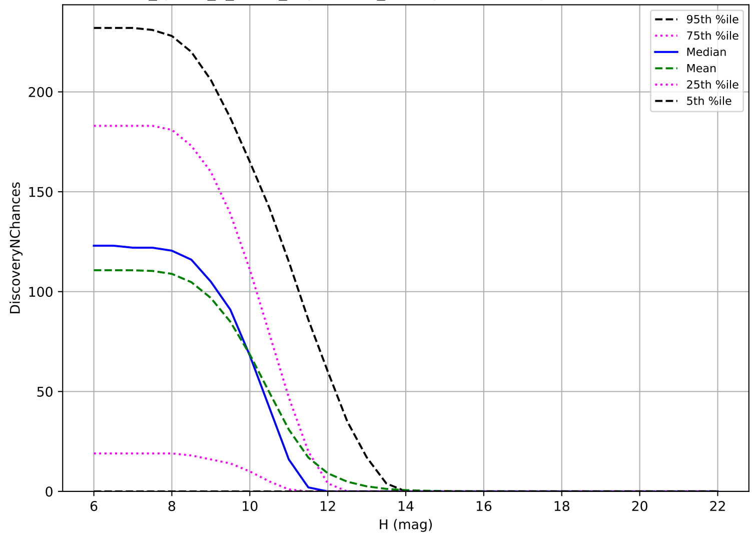
too_ignore_5_1v3.4_10yrs: OCC_r20 3 pairs in 15 nights detection loss
