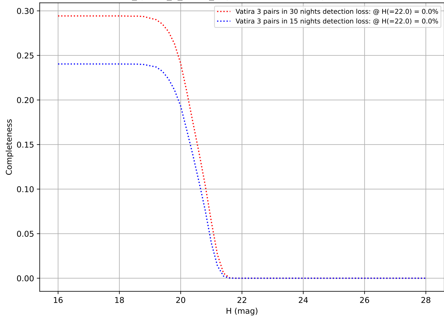
too_ignore_5_1v3.4_10yrs: DifferentialCompleteness
