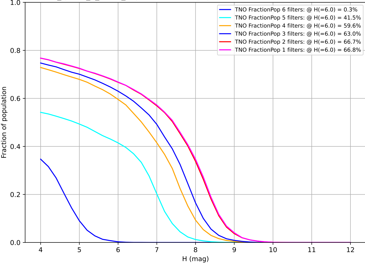
too_ignore_5_1v3.4_10yrs: Fraction of population with colors in X filters TNO
