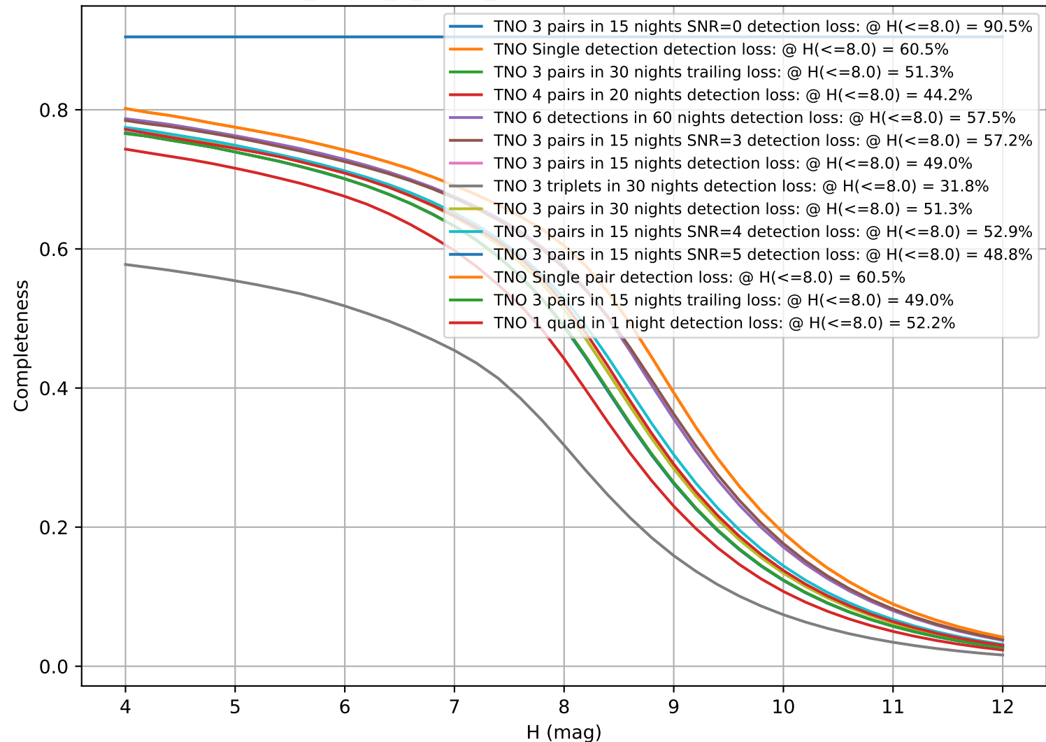
too_ignore_5_1v3.4_10yrs: CumulativeCompleteness
