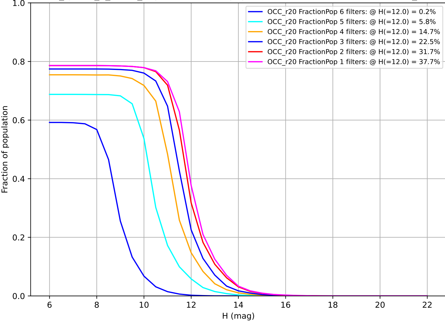
too_ignore_5_1v3.4_10yrs: Fraction of population with colors in X filters OCC_r20
