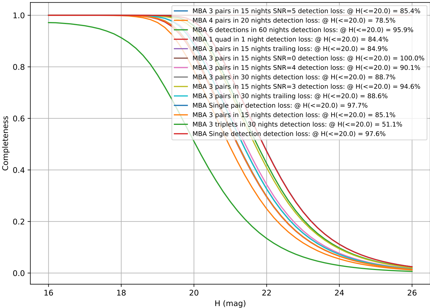
too_ignore_5_1v3.4_10yrs: CumulativeCompleteness
