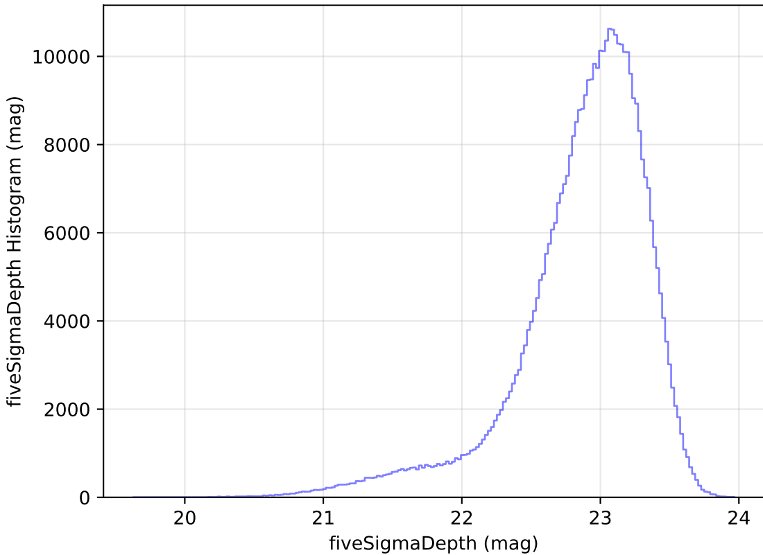
too_ignore_5_1v3.4_10yrs z: fiveSigmaDepth Histogram
