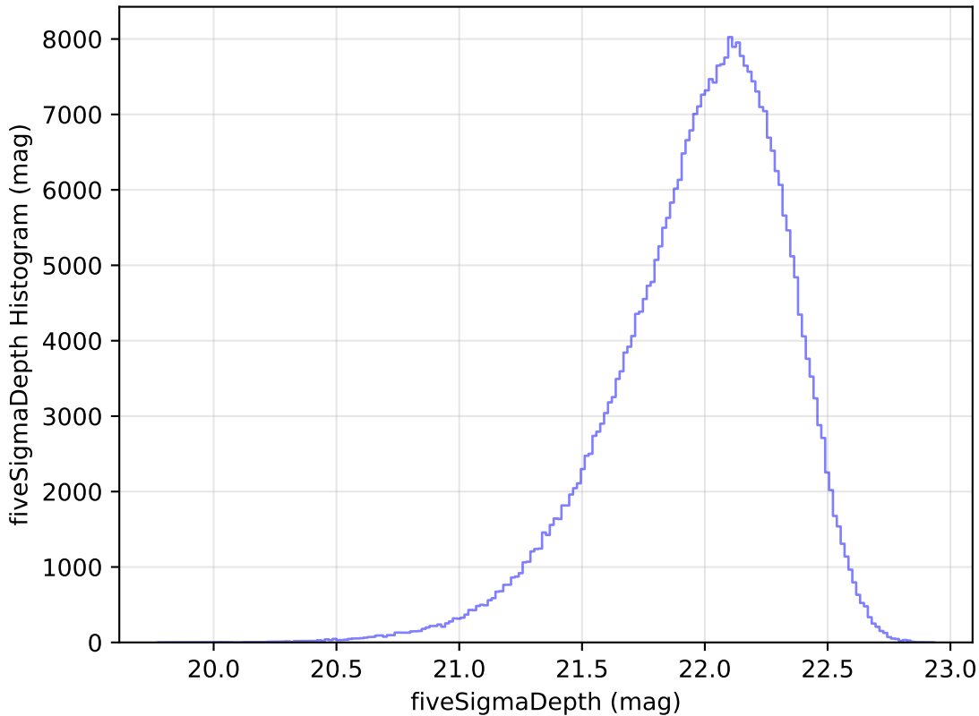
too_ignore_5_1v3.4_10yrs y: fiveSigmaDepth Histogram
