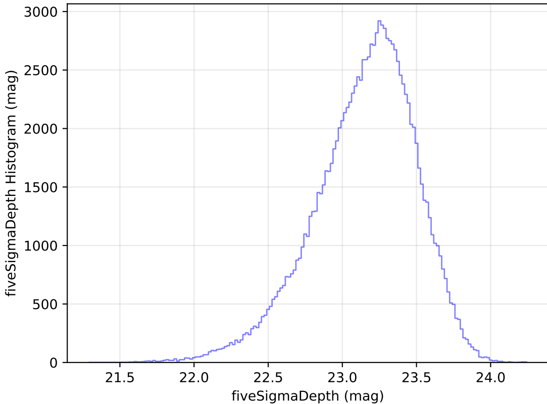
too_ignore_5_1v3.4_10yrs u: fiveSigmaDepth Histogram
