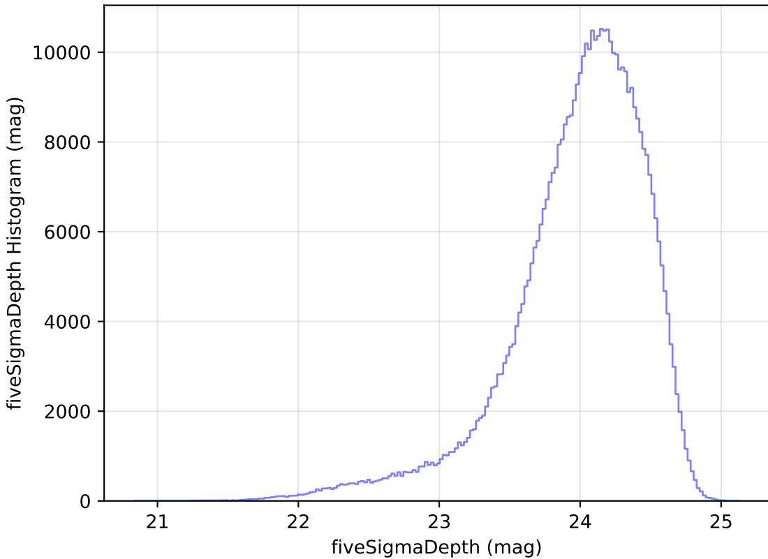
too_ignore_5_1v3.4_10yrs r: fiveSigmaDepth Histogram
