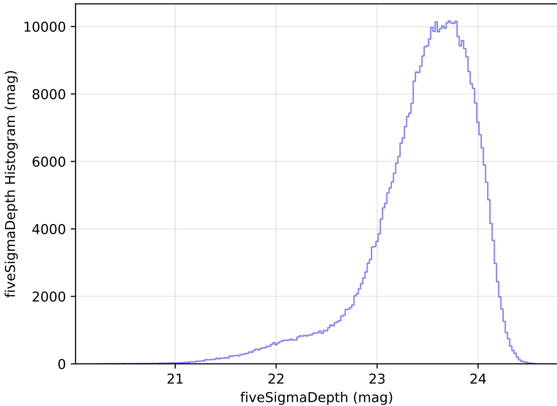
too_ignore_5_1v3.4_10yrs i: fiveSigmaDepth Histogram
