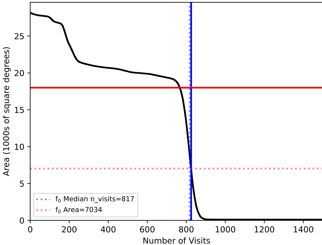
too_ignore_5_1v3.4_10yrs : f0
