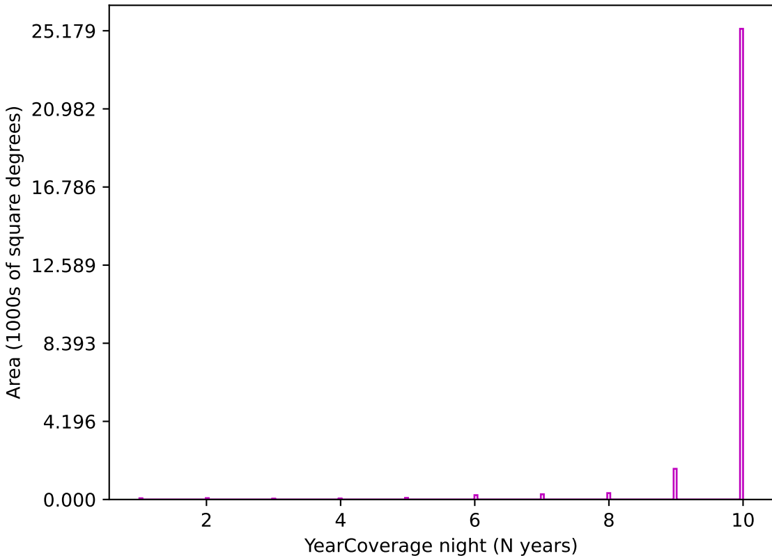
too_ignore_5_1v3.4_10yrs z band: YearCoverage night
