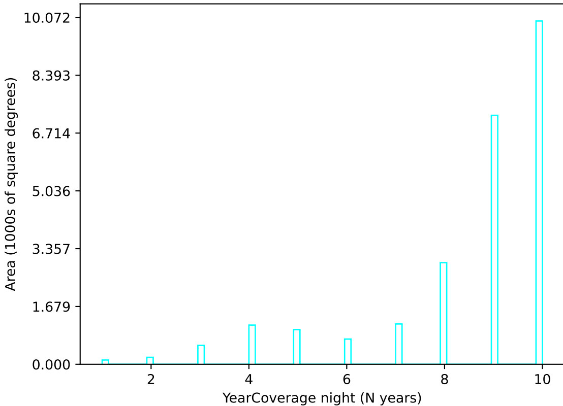
too_ignore_5_1v3.4_10yrs u band: YearCoverage night
