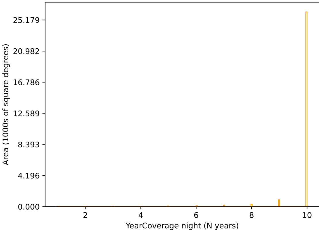
too_ignore_5_1v3.4_10yrs r band: YearCoverage night
