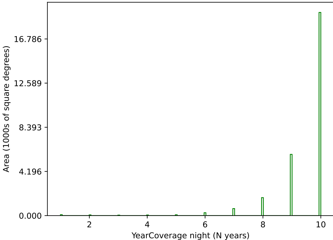
too_ignore_5_1v3.4_10yrs g band: YearCoverage night
