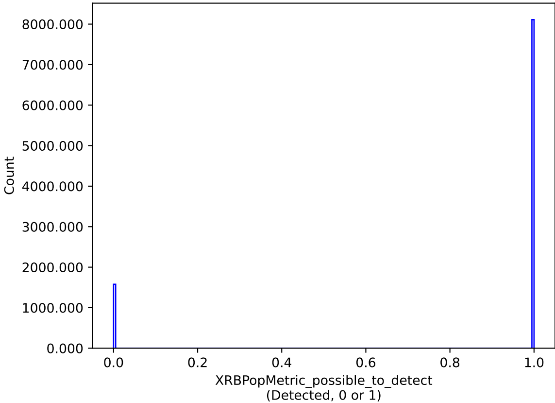
too_ignore_5_1v3.4_10yrs : XRBPoMetric_possible_to_detect
