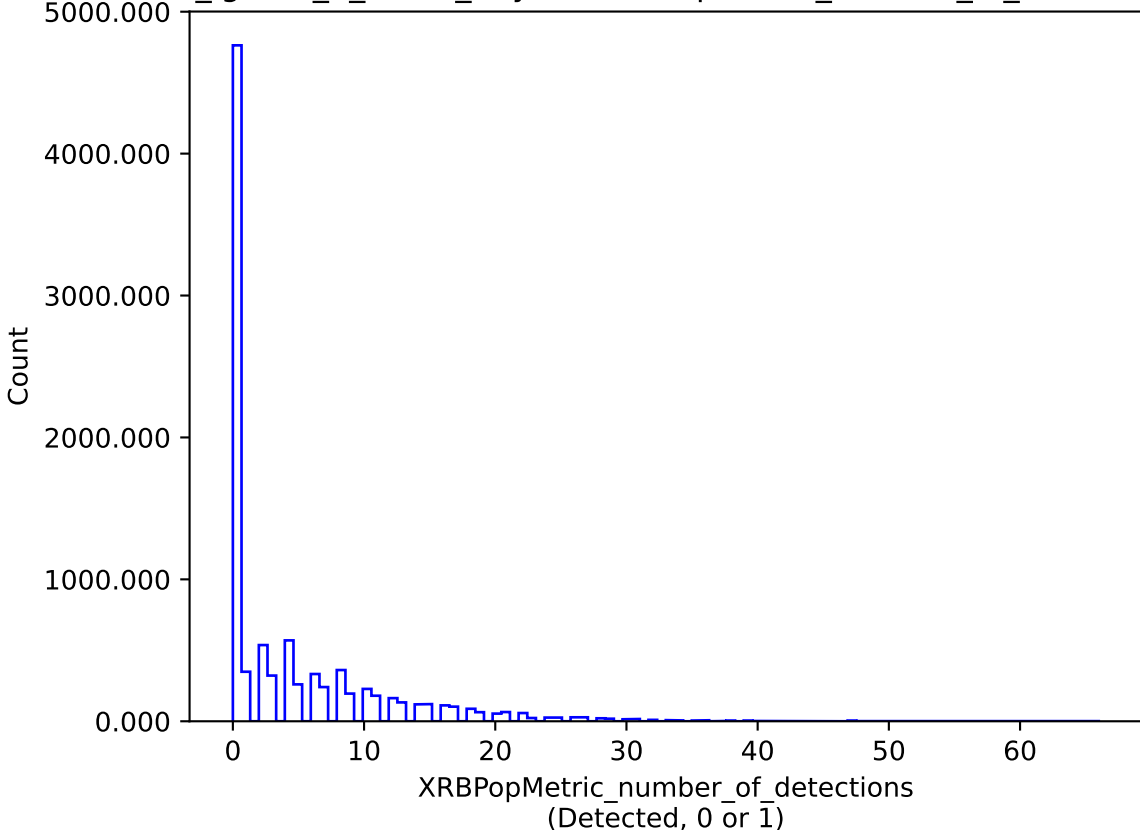
too_ignore_5_1v3.4_10yrs : XRBPopMetric_number_of_detections
