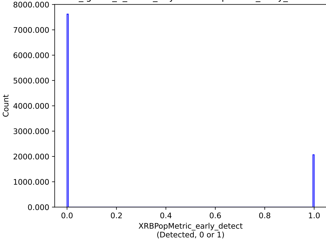
too_ignore_5_1v3.4_10yrs : XRBPoMetric_early_detect
