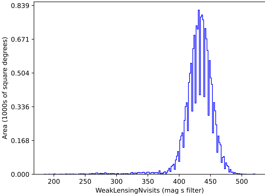
too_ignore_5_1v3.4_10yrs gri band non-DD: WeakLensingNvisits
