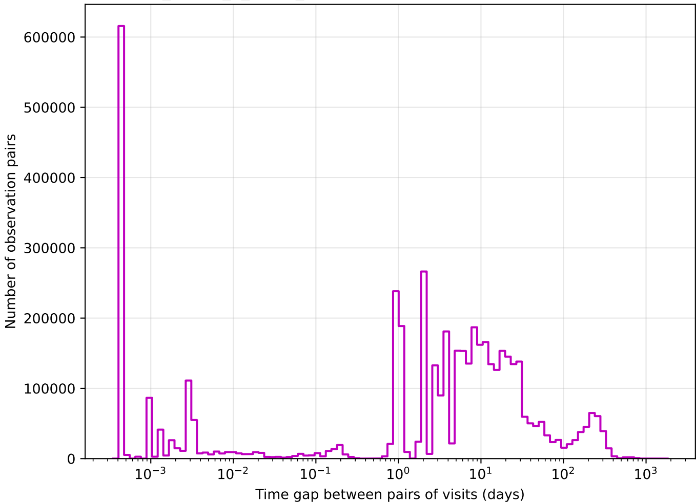
too_ignore_5_1v3.4_10yrs z band: Tgaps observationStartMJD
