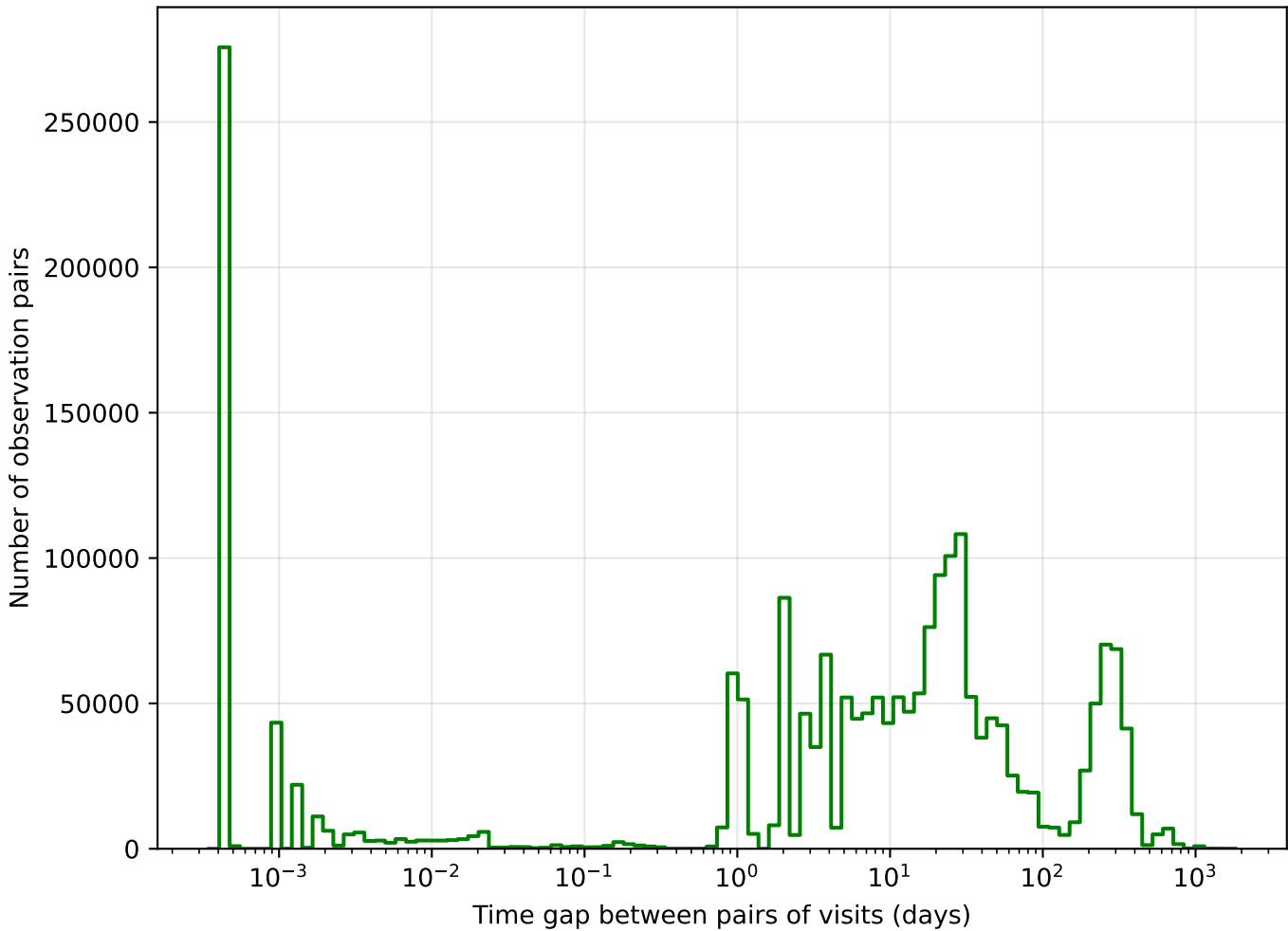
too_ignore_5_1v3.4_10yrs g band: Tgaps observationStartMJD
