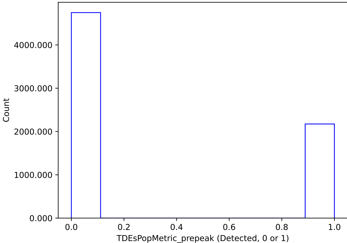
too_ignore_5_1v3.4_10yrs : TDEsPopMetric_prepeak
