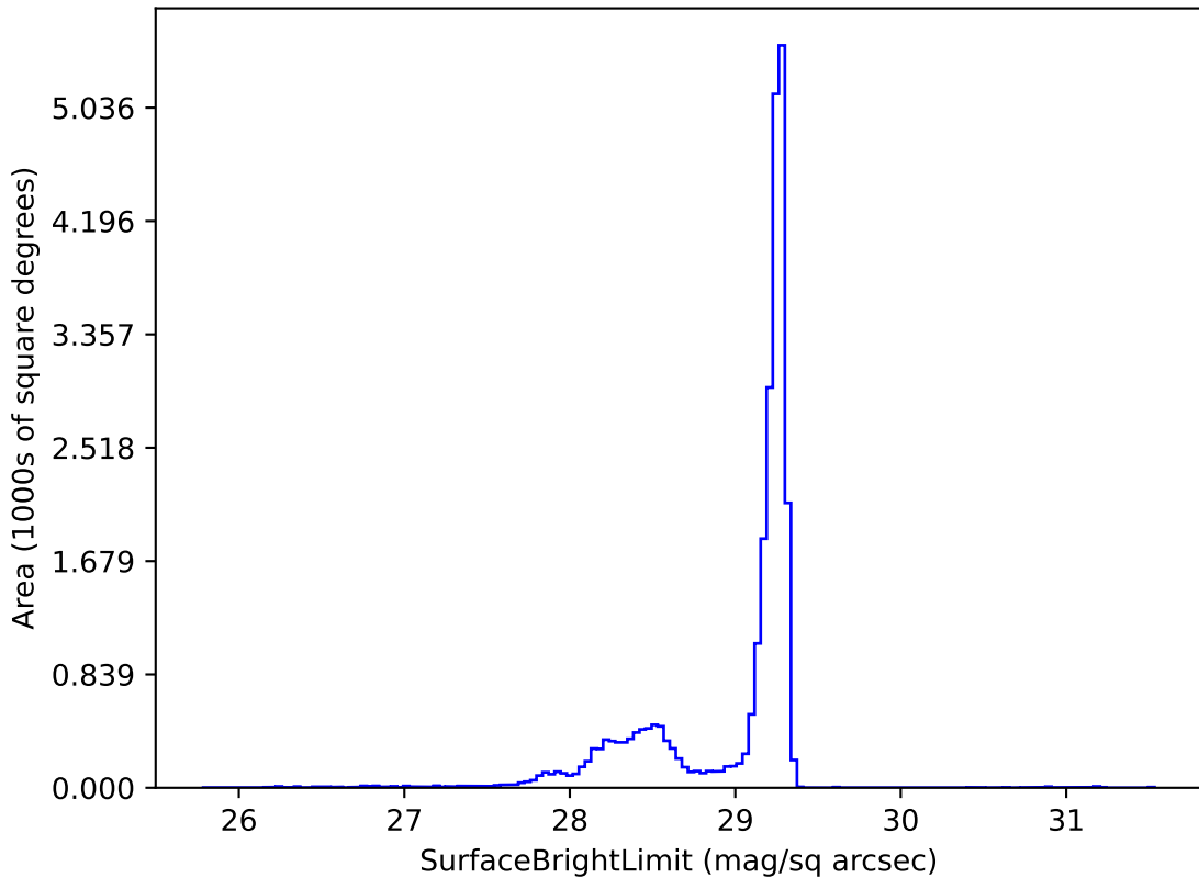
too_ignore_5_1v3.4_10yrs z: SurfaceBrightLimit
