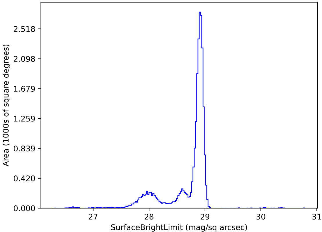
too_ignore_5_1v3.4_10yrs u: SurfaceBrightLimit
