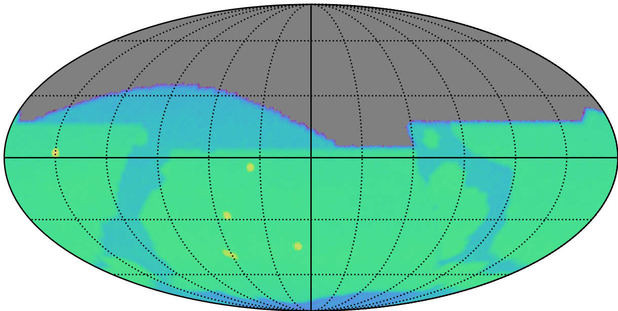
too_ignore_5_1v3.4_10yrs r: SurfaceBrightLimit
