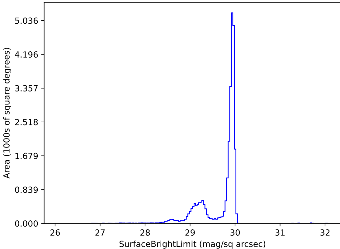
too_ignore_5_1v3.4_10yrs i: SurfaceBrightLimit
