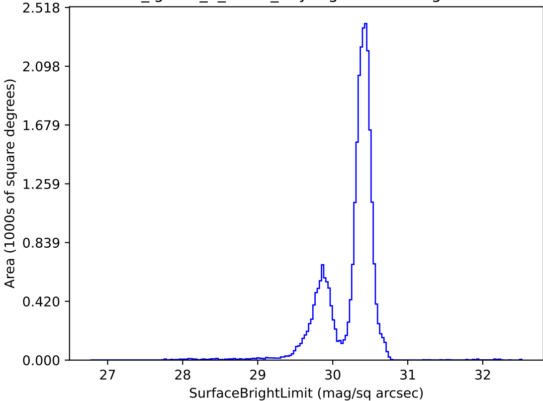
too_ignore_5_1v3.4_10yrs g: SurfaceBrightLimit
