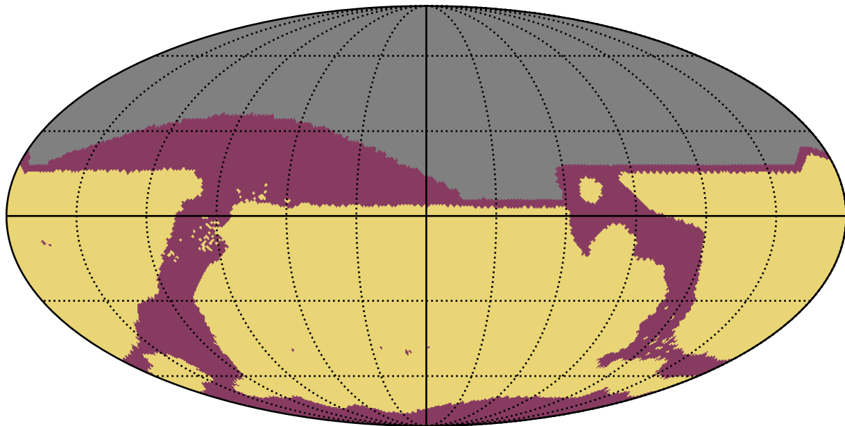
too_ignore_5_1v3.4_10yrs : RapidRevisits
