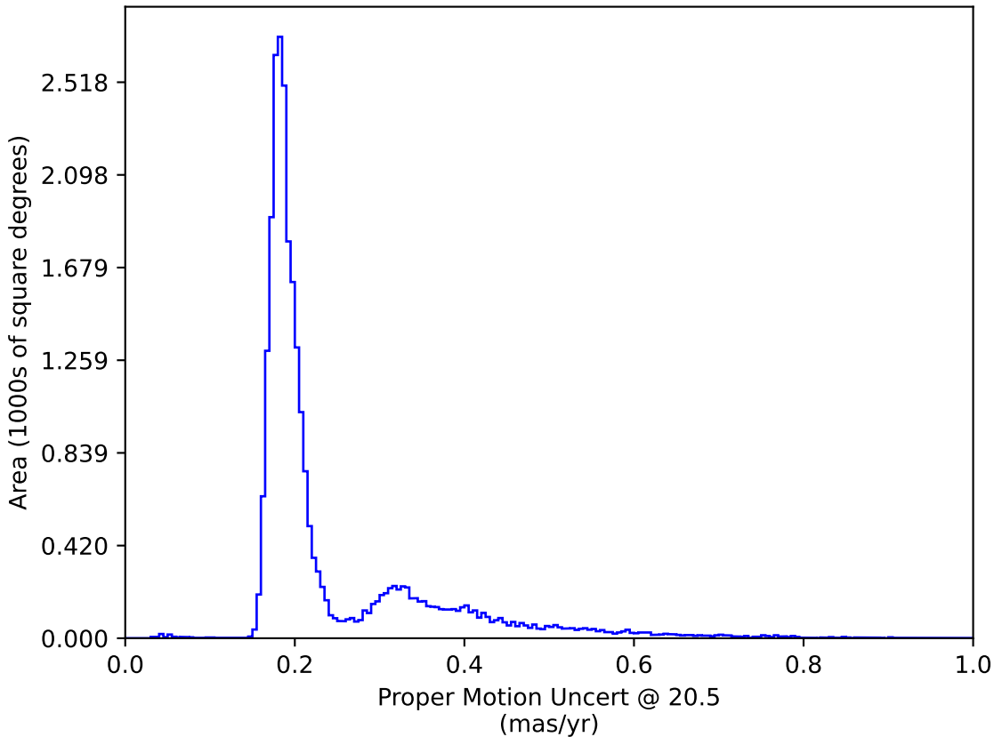
too_ignore_5_1v3.4_10yrs : Proper Motion Uncert @ 20.5
