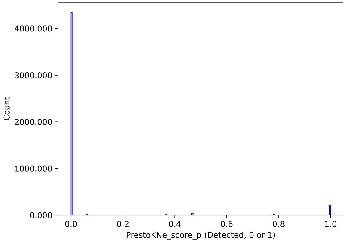
too_ignore_5_1v3.4_10yrs : PrestoKNe_score_p
