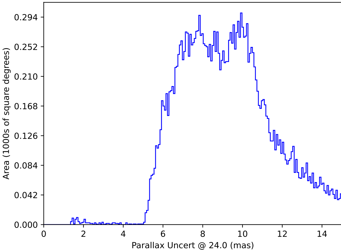
too_ignore_5_1v3.4_10yrs : Parallax Uncert @ 24.0
