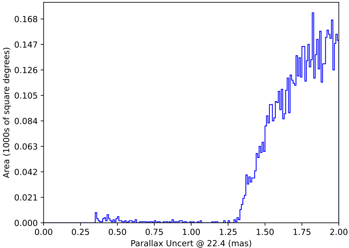
too_ignore_5_1v3.4_10yrs : Parallax Uncert @ 22.4
