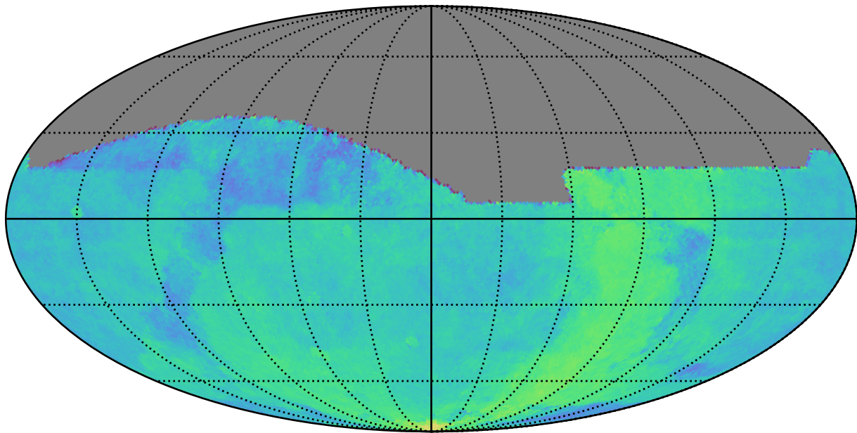
too_ignore_5_1v3.4_10yrs : Parallax Coverage @ 24.0
