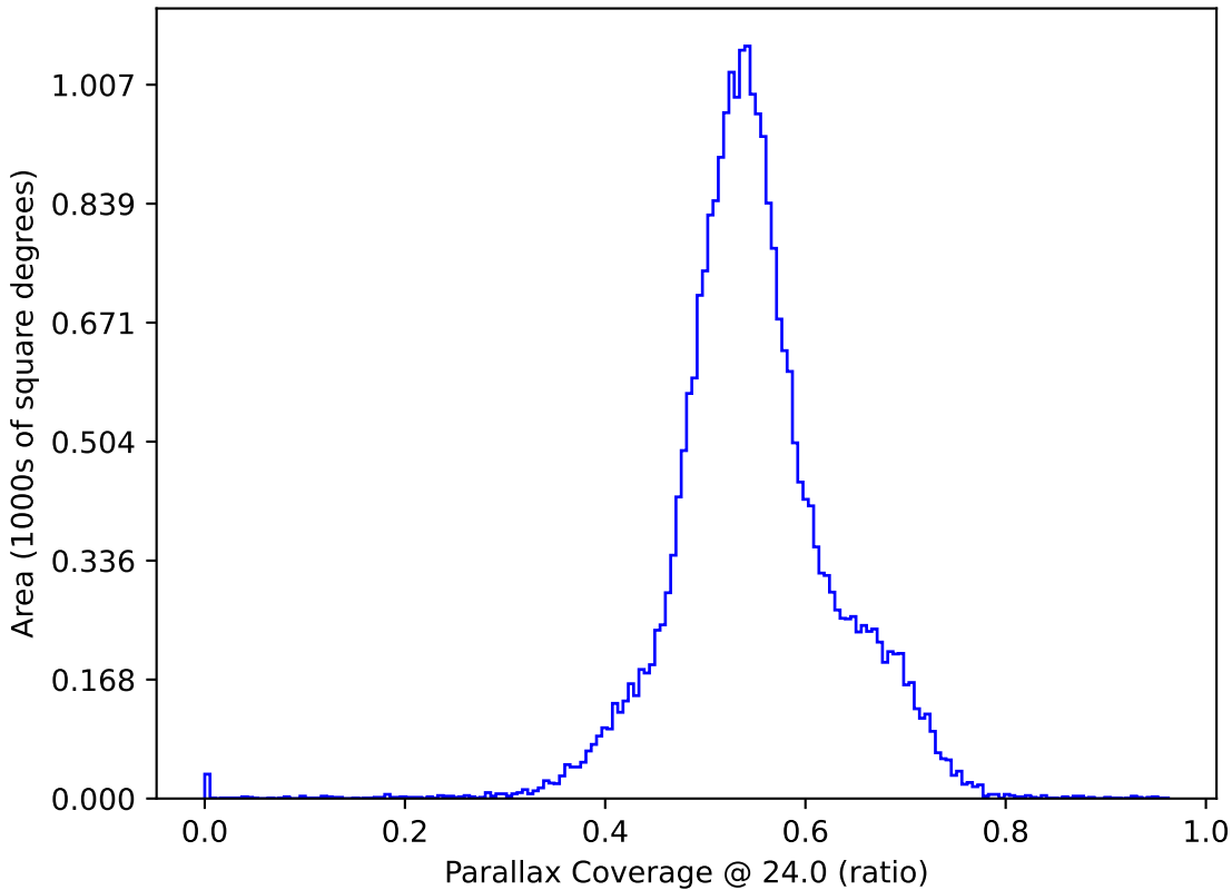
too_ignore_5_1v3.4_10yrs : Parallax Coverage @ 24.0
