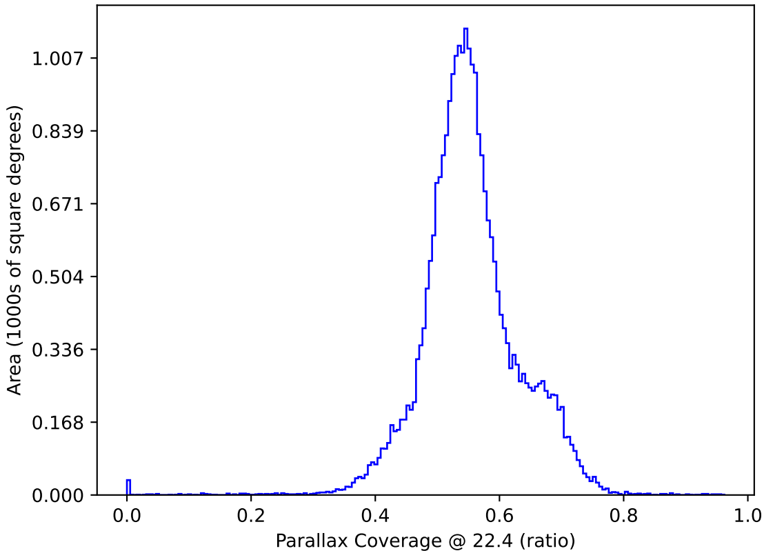
too_ignore_5_1v3.4_10yrs : Parallax Coverage @ 22.4
