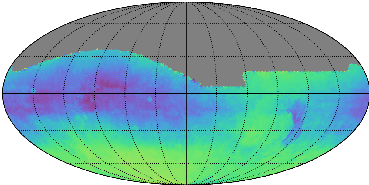
too_ignore_5_1v3.4_10yrs : Parallax-DCR degeneracy @ 24.0
