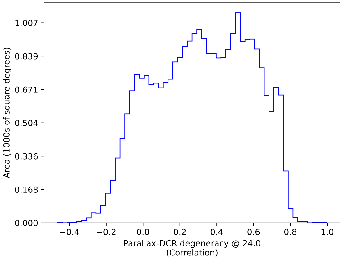
too_ignore_5_1v3.4_10yrs : Parallax-DCR degeneracy @ 24.0
