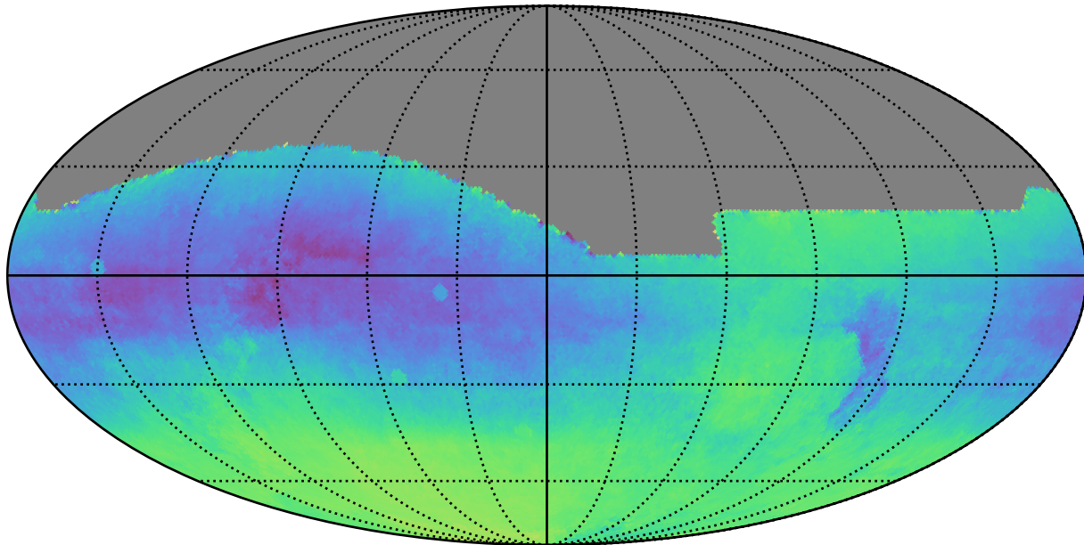
too_ignore_5_1v3.4_10yrs : Parallax-DCR degeneracy @ 22.4
