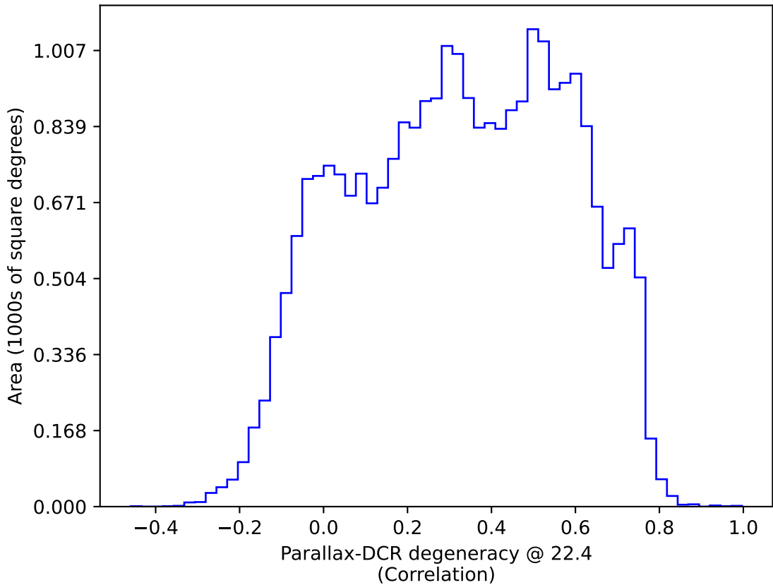
too_ignore_5_1v3.4_10yrs : Parallax-DCR degeneracy @ 22.4
