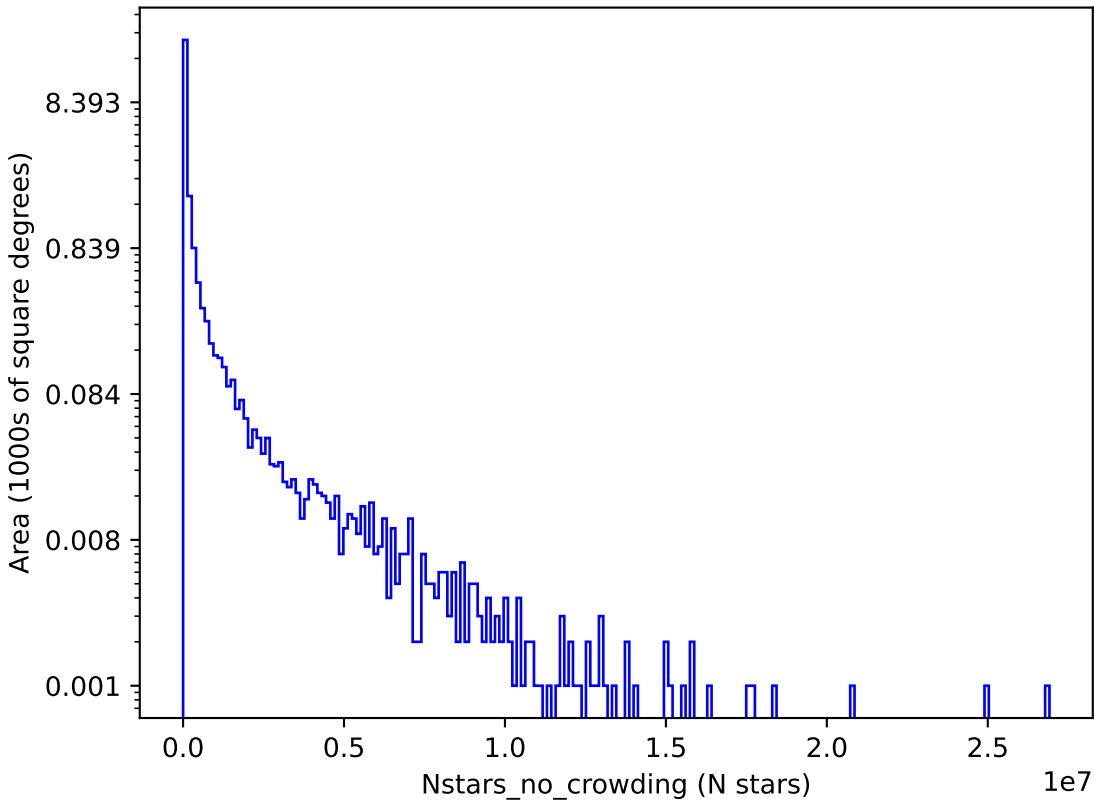
too_ignore_5_1v3.4_10yrs z: Nstars_no_crowding
