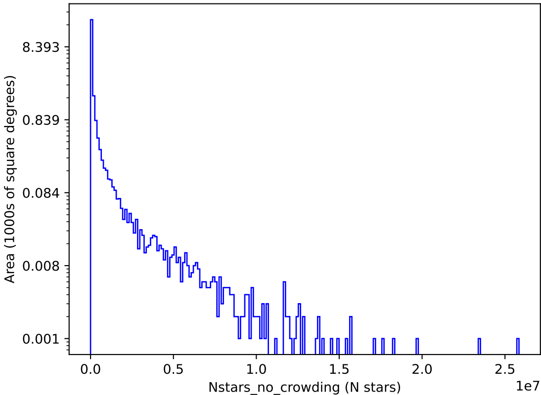
too_ignore_5_1v3.4_10yrs y: Nstars_no_crowding
