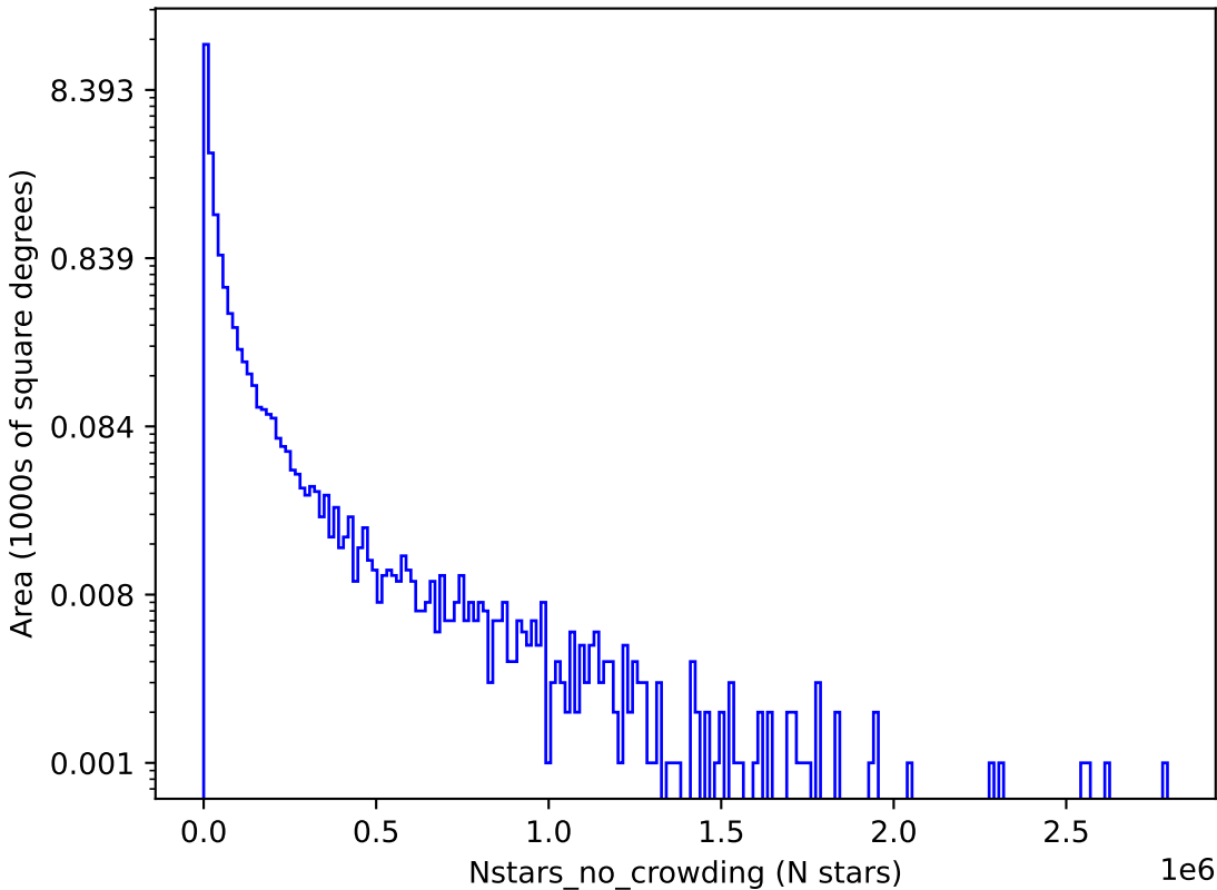
too_ignore_5_1v3.4_10yrs u: Nstars_no_crowding
