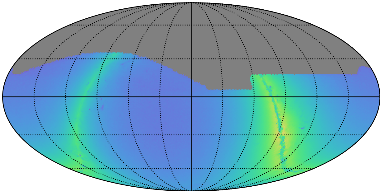
too_ignore_5_1v3.4_10yrs i: Nstars_no_crowding
