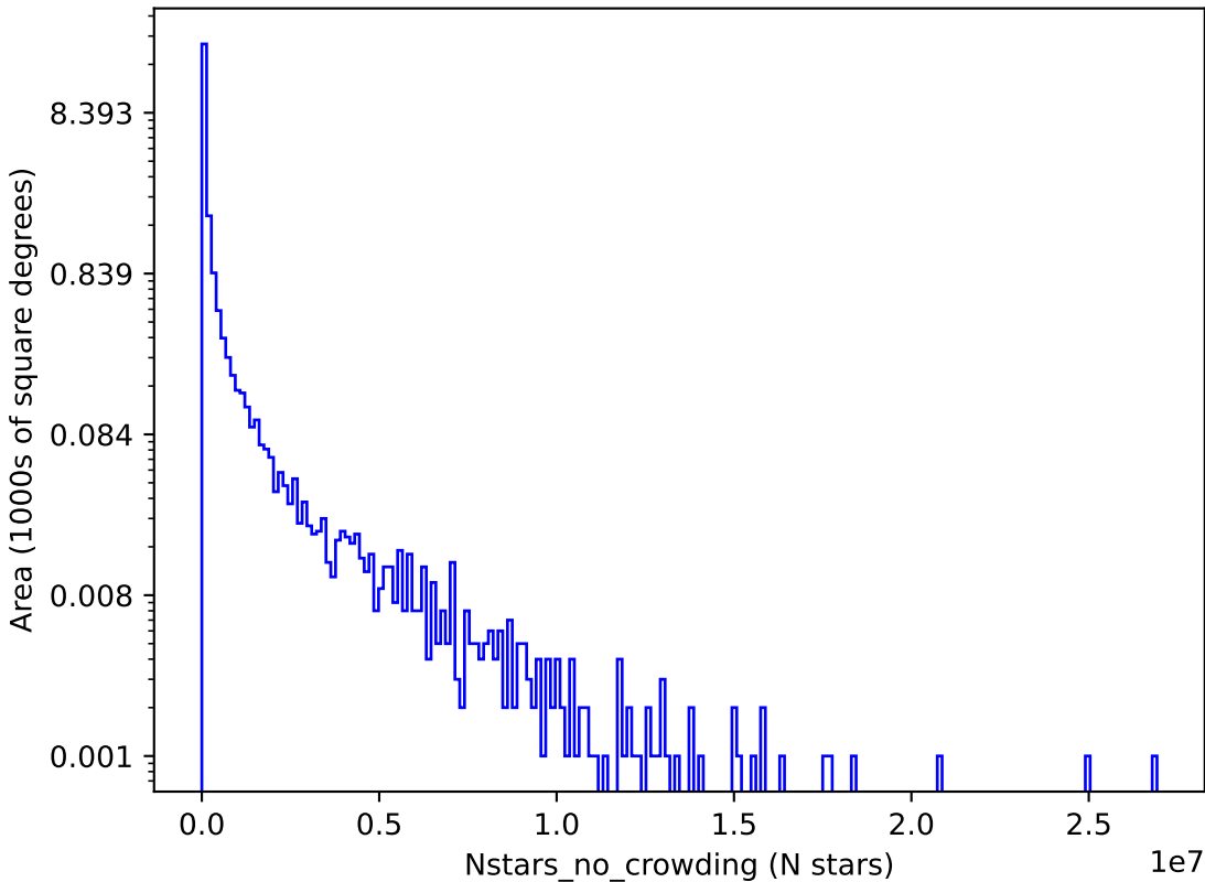
too_ignore_5_1v3.4_10yrs i: Nstars_no_crowding
