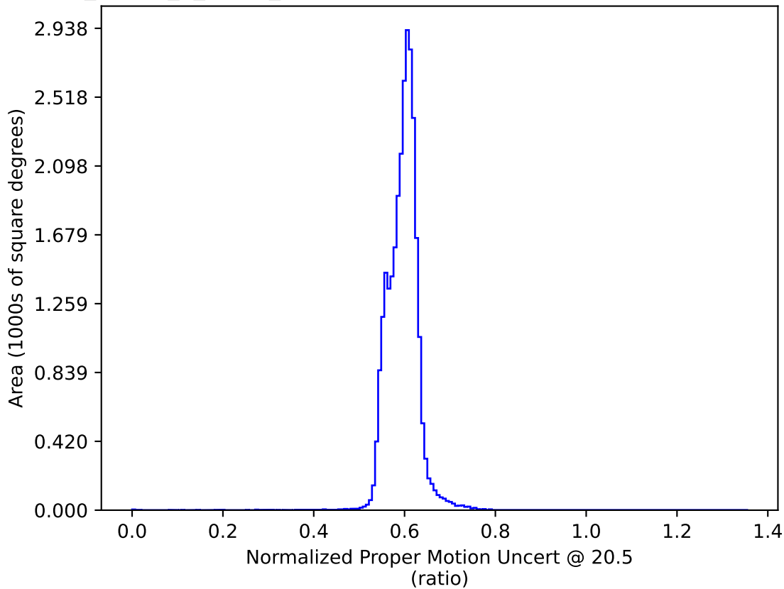
too_ignore_5_1v3.4_10yrs : Normalized Proper Motion Uncert @ 20.5
