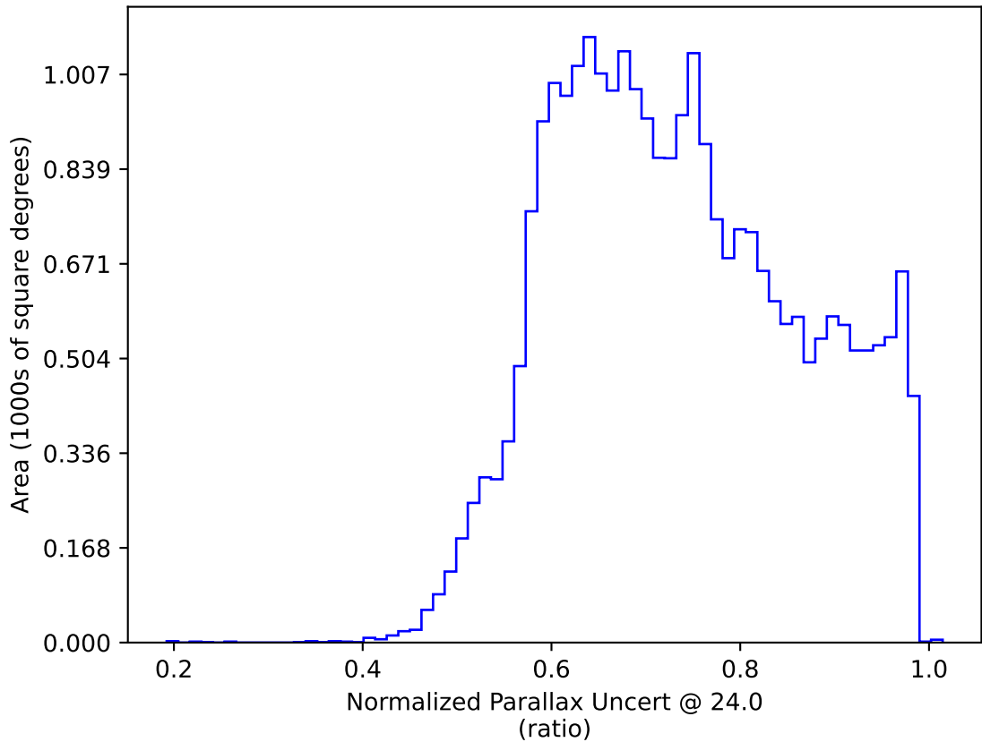
too_ignore_5_1v3.4_10yrs : Normalized Parallax Uncert @ 24.0
