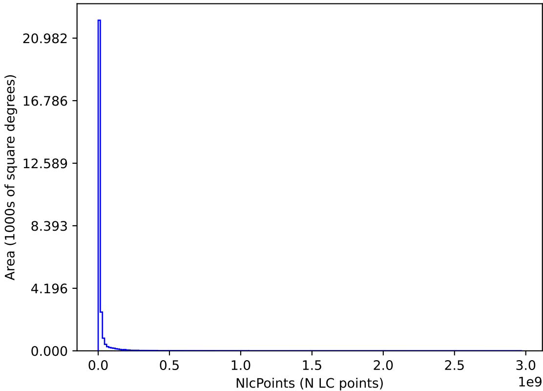
too_ignore_5_1v3.4_10yrs : NlcPoints
