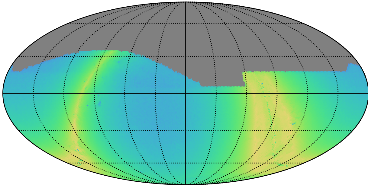
too_ignore_5_1v3.4_10yrs z: N stars to Precision 0.20
